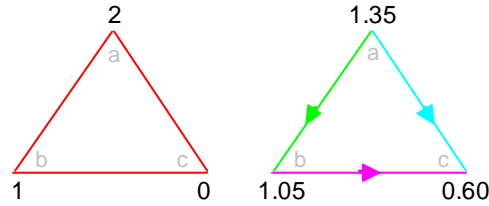
FIGURE 11: On the left endowments, on the right Cournot outcomes.
