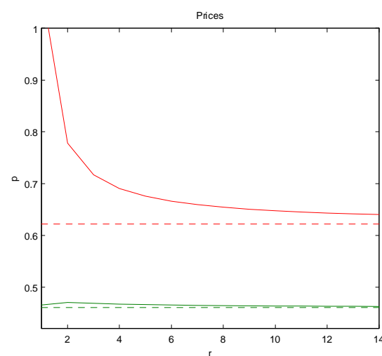
FIGURE 10B: On the vertical axis prices on the horizontal axis the replica
