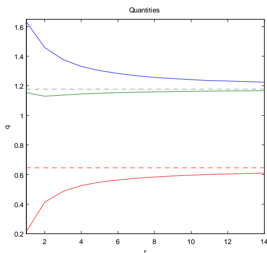
FIGURE 10A: On the vertical axis consumption on the horizontal axis the replica
