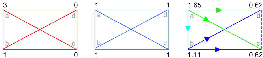
FIGURE 1: On the left the economy, at the center efficiency, on the right Cournot outcomes. Edges on which no flow transits are dashed.
