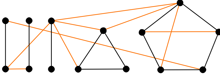
FIGURE 4. A network that can be covered by a match and odd cycles disjoint union
