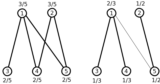
FIGURE 1. Networks G_1 (left) and G_2
