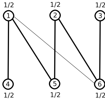
FIGURE 5. Network G_5
