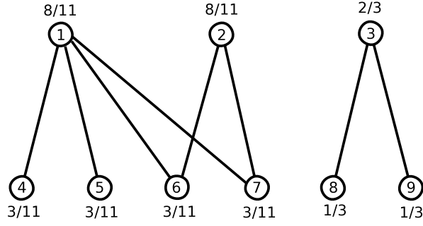
FIGURE 6. Network G_3^*(p)
