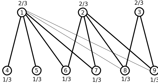
FIGURE 2. Network G_3
