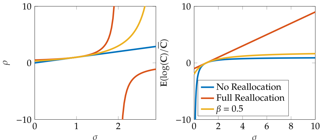
Figure 2: The left panel plots the macro elasticity of substitution \rho against the structural elasticity of substitution \sigma for the model from Proposition 4.1. The second panel plots expected log GDP relative to its certainty equivalent, in units of variance, as a function of the structural elasticity of substitution for the same model.
